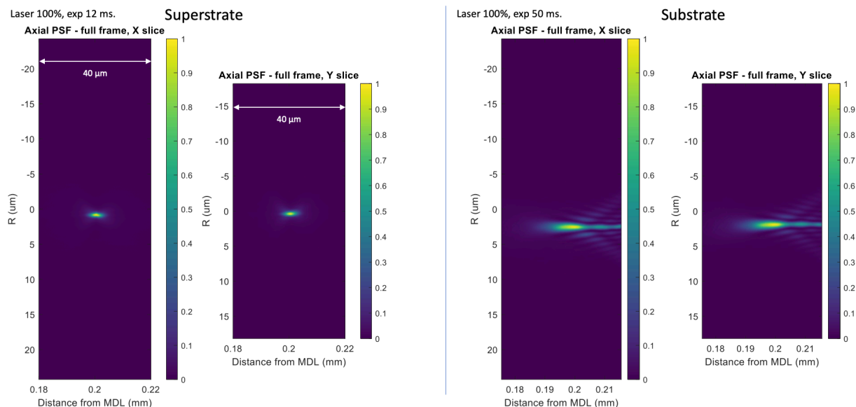
Fig. S7.5 Measured axial PSF full frame data. Scan length: \pm 20 \mu\text{m} on either side of best focal plane, Total length = 40 \mu\text{m} , Step size = 0.1 \mu\text{m} , Number of steps = 400, \lambda = 634 \text{ nm} , \text{bw} = 5 \text{ nm} (set using VARIA).
