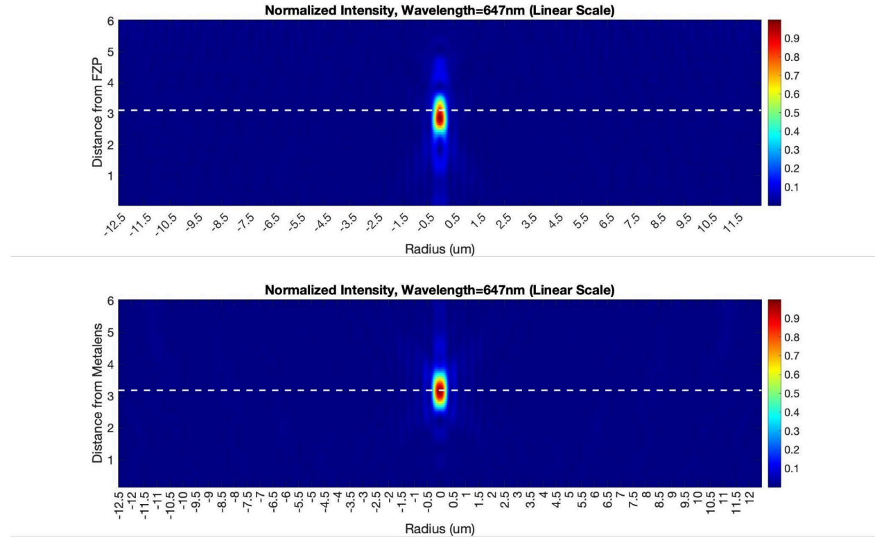
Fig S1.19: Simulated PSF in the XZ plane for the FZP (top) Metalens FZP (bottom) with diameter = 25 \mu\text{m} , and incidence from substrate. Note that the metalens outperformed the FZP in focusing efficiency (FZP at 3.5% compared to the metalens at 11%).
