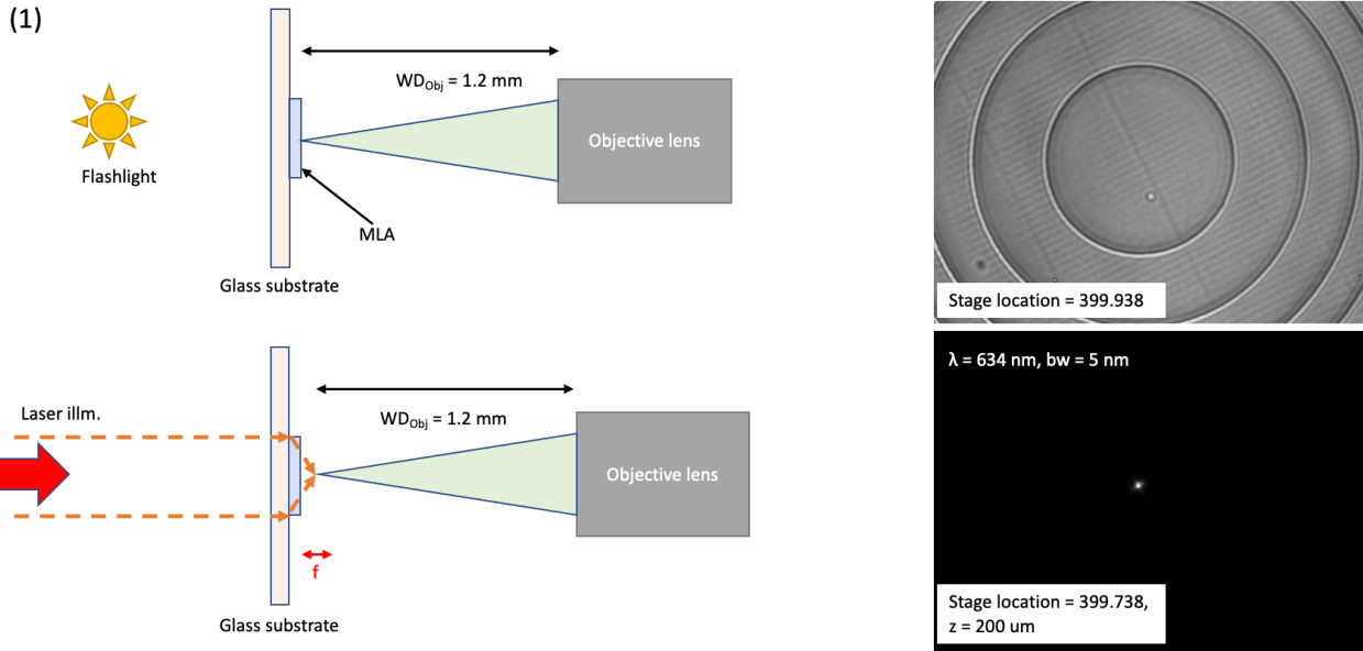
Fig. S7.2 Experimental setup for illumination from superstrate (+Z direction). First, the MLA is brought in focus of the Objective lens by illuminating from behind using LED flashlight. Patterned side faces measurement setup. Next, the Objective is moved back by the expected focal length to search for the PSF. In this case, the flashlight is removed and the collimated superK laser illumination is incident on the sample.
