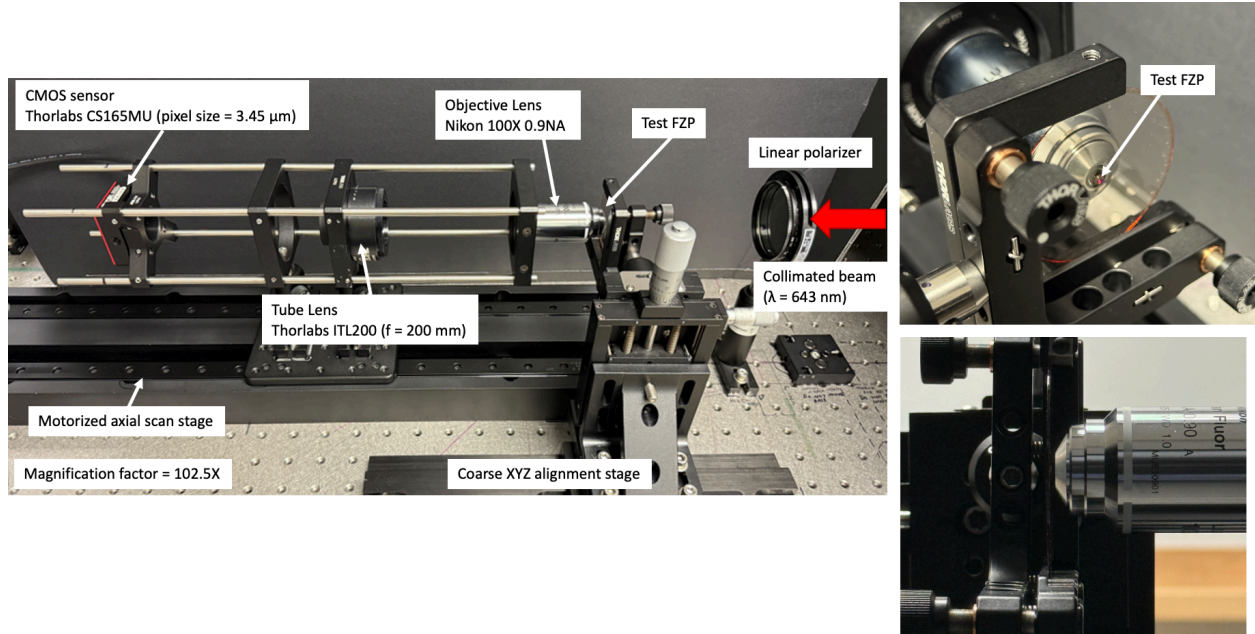
Fig. S7.1 Experimental setup for magnification of the PSF of the FZP.
