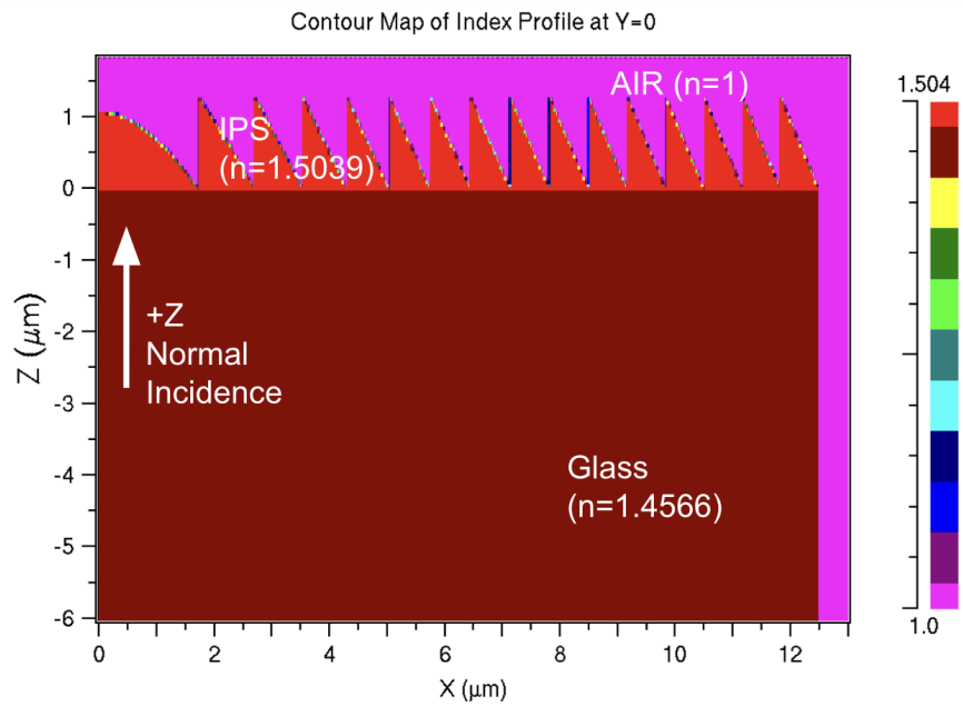
Fig S1.12: Material Profiles of Metalens (a) and FZP (b) with diameter = 25\mu\text{m} , and focal length = 2.67\mu\text{m} with glass substrate.
