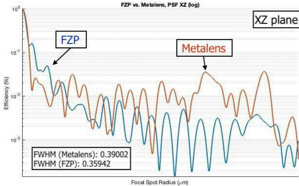
Fig S1.16: Simulated PSF in the XZ plane for the FZP (top) and Metalens (bottom) with diameter = 25\mu\text{m} , focal length = 17\mu\text{m} , and incidence from air. Note that the efficiency of the FZP is 16%, compared to the metalens at 5%.
