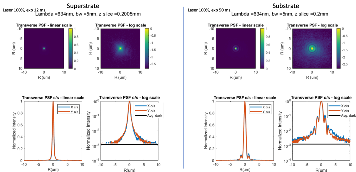
Fig. S7.10 Measured transverse PSFs. Scan length: \pm 20 \mu\text{m} on either side of best focal plane, Total length = 40 \mu\text{m} , Step size = 0.1 \mu\text{m} , Number of steps = 400, \lambda = 634 \text{ nm} , \text{bw} = 5 \text{ nm} (set using VARIA).
