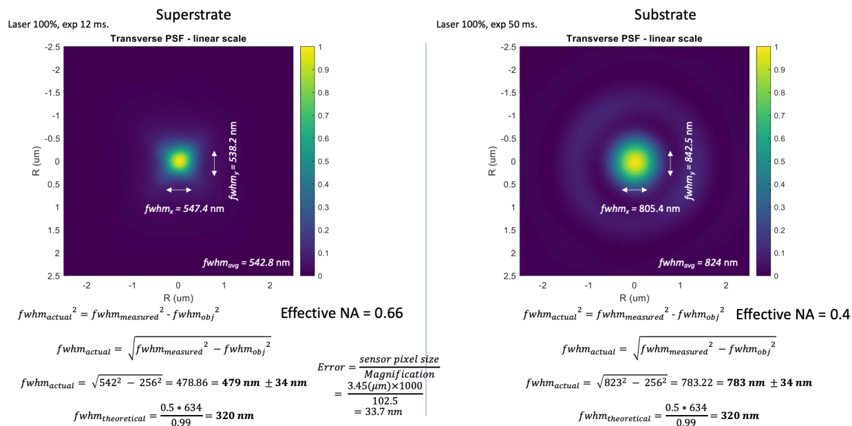
Fig. S7.11 Estimating FWHM in both directions of incidence.
