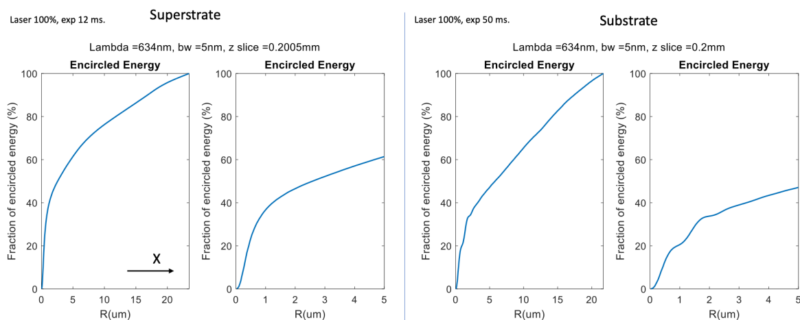
Fig. S7.12 Measured encircled energy for both directions of incidence.
