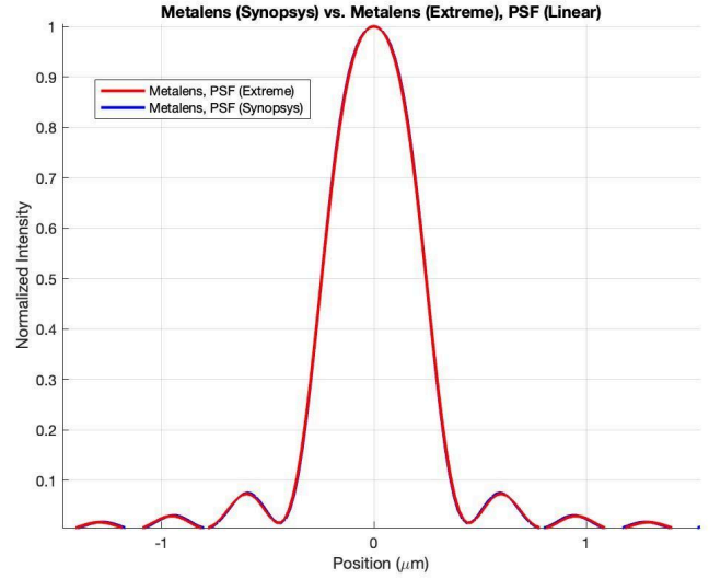
Fig S1.6: Validation results. (a) Metalens results from simulation on a machine with 60 cores and 2 TB of RAM (Local) vs. results from simulation on a machine with 16 cores and 120 GB of RAM (Synopsis). (b) FZP simulation results from different FDTD softwares (RSoft vs. MEEP). (c) Encircled energy comparison demonstrating equivalence in Local vs. Synopsis simulations. (d) Point Spread Function plot comparison demonstrating equivalence in Local vs. Synopsis simulations.
