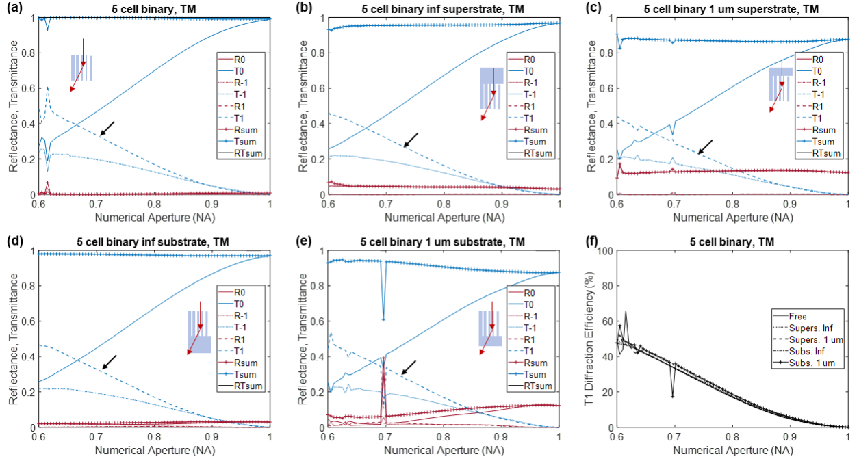
Fig. S3.12: Simulation results for TM illumination showing all transmission and diffraction orders vs NA for 5-cell binary blazed grating for (a) free grating, (b) infinite superstrate, (c) finite superstrate, (d) infinite substrate, and (e) finite substrate cases. The first transmitted order is pointed out by the black arrow. (f) First-order transmission diffraction efficiency for the 5 cases, extracted from (a-e). We noted the presence of \pm 2^{\text{nd}} reflected and transmitted orders for \text{NA} < 0.8 in (b) and (d) respectively, but they have not been plotted here.
