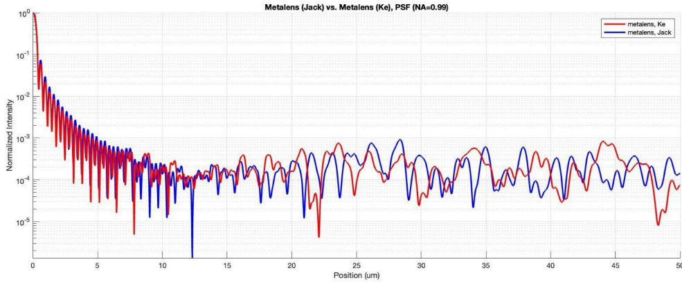
Fig S1.2: Figures comparing metalens designs: (a) Encircled energy comparison in the XZ plane between two lenses of varying period. The lens with smaller period = 0.3\ \mu\text{m} demonstrated a higher efficiency. (b) Point Spread function comparison in the XZ plane. Similarly, the lens with smaller period = 0.3\ \mu\text{m} demonstrated a higher efficiency though FWHM was equal for both.
