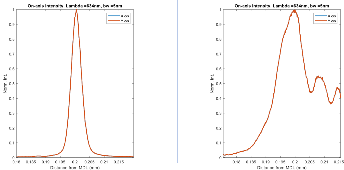
Fig. S7.6 Measured on-axis PSF data. Scan length: \pm 20 \mu\text{m} on either side of best focal plane, Total length = 40 \mu\text{m} , Step size = 0.1 \mu\text{m} , Number of steps = 400, \lambda = 634 \text{ nm} , \text{bw} = 5 \text{ nm} (set using VARIA).
