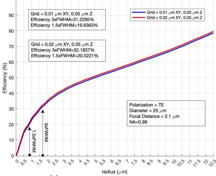
FZP, Simulation Grid Size Comparison (Encircled Energy)
