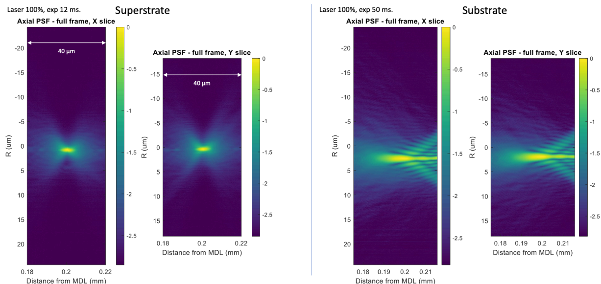
Fig. S7.7 Measured axial PSF data, full-frame log scale. Scan length: \pm 20 \mu\text{m} on either side of best focal plane, Total length = 40 \mu\text{m} , Step size = 0.1 \mu\text{m} , Number of steps = 400, \lambda = 634 \text{ nm} , \text{bw} = 5 \text{ nm} (set using VARIA).
