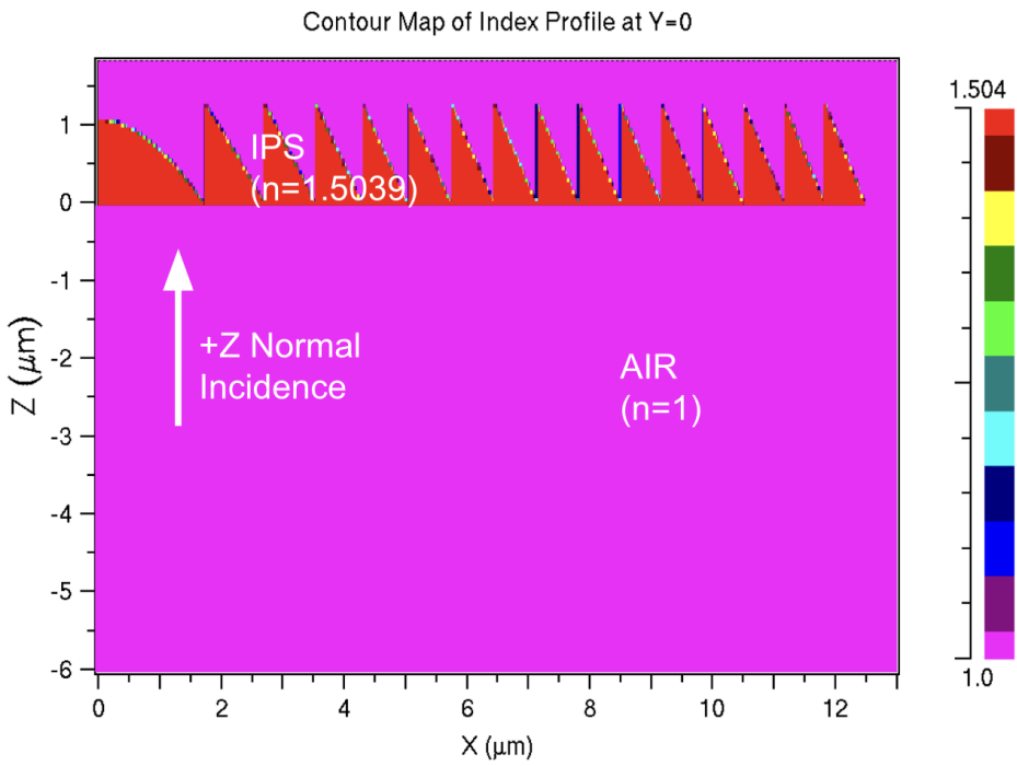
Fig S1.21: Material Profiles of Metalens (a) and FZP (b) with diameter = 25\mu\text{m} , and focal length = 2.67\mu\text{m} without substrate.
