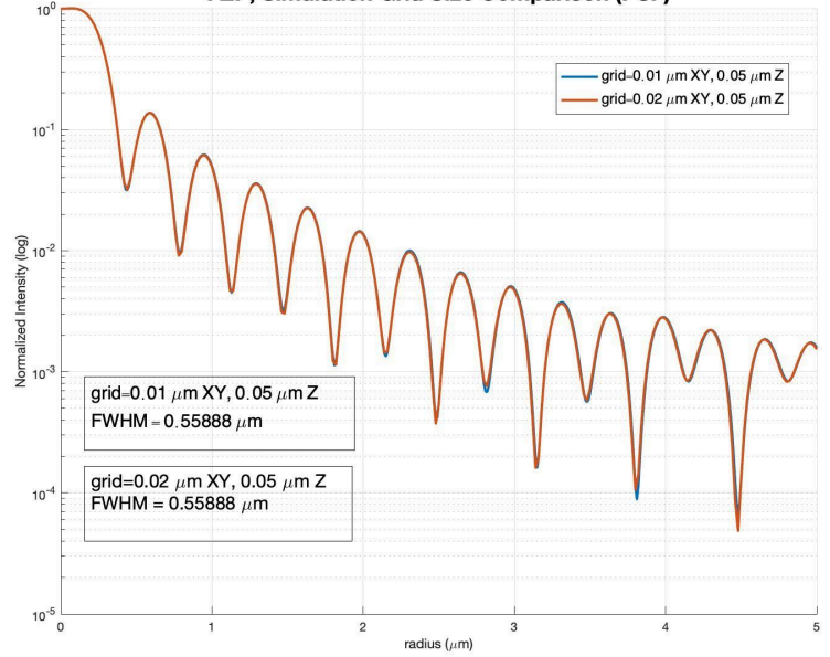
FZP, Simulation Grid Size Comparison (PSF)
