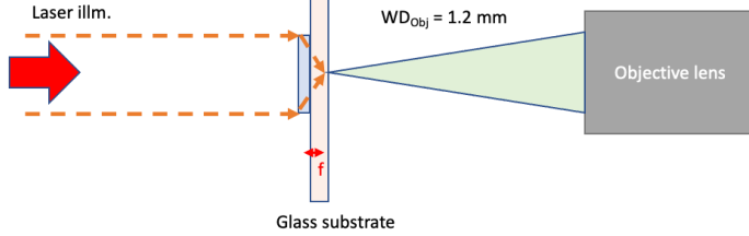
Fig. S7.3 Experimental setup for illumination from substrate (-Z direction). First, the MLA is brought in focus of the Objective lens by illuminating from behind using LED flashlight. Focusing is performed through the glass surface. Patterned side faces incident illumination. Next, the Objective is moved back by the expected focal length to search for the PSF. In this case, the flashlight is removed and the collimated superK laser illumination is incident on the sample.
