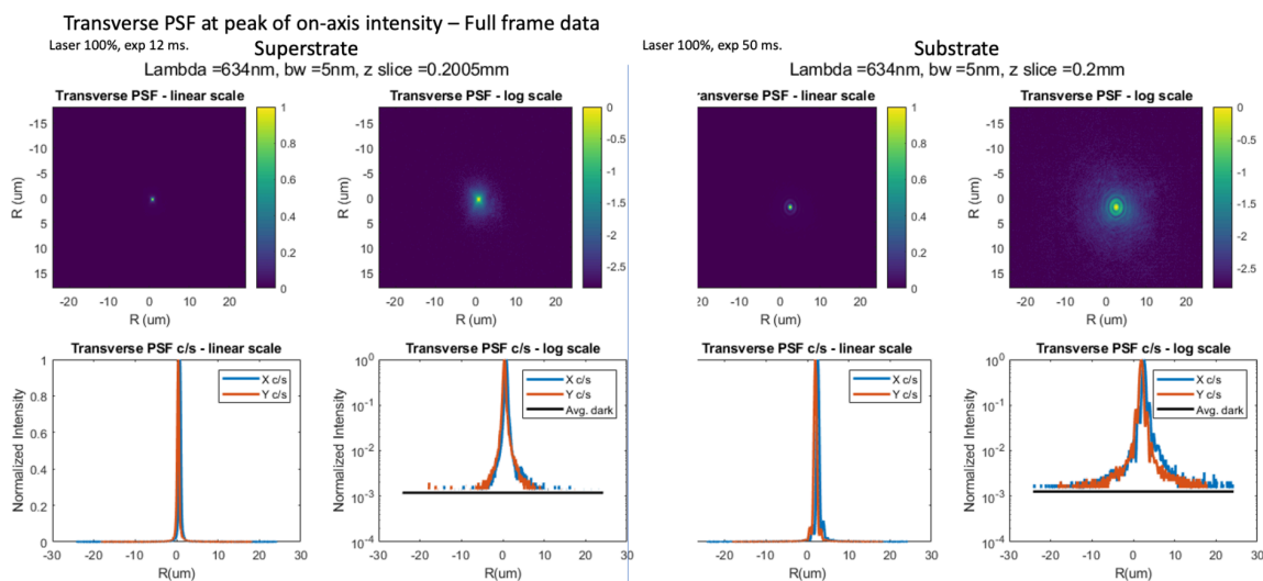
Fig. S7.8 Measured transverse PSFs at peak on-axis intensity location.
