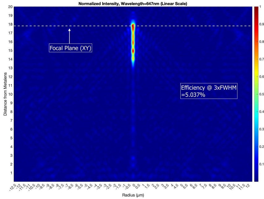
Fig S1.16: Simulated PSF in the XZ plane for the FZP (top) and Metalens (bottom) with diameter = 25\mu\text{m} , focal length = 17\mu\text{m} , and incidence from air. Note that the efficiency of the FZP is 16%, compared to the metalens at 5%.
