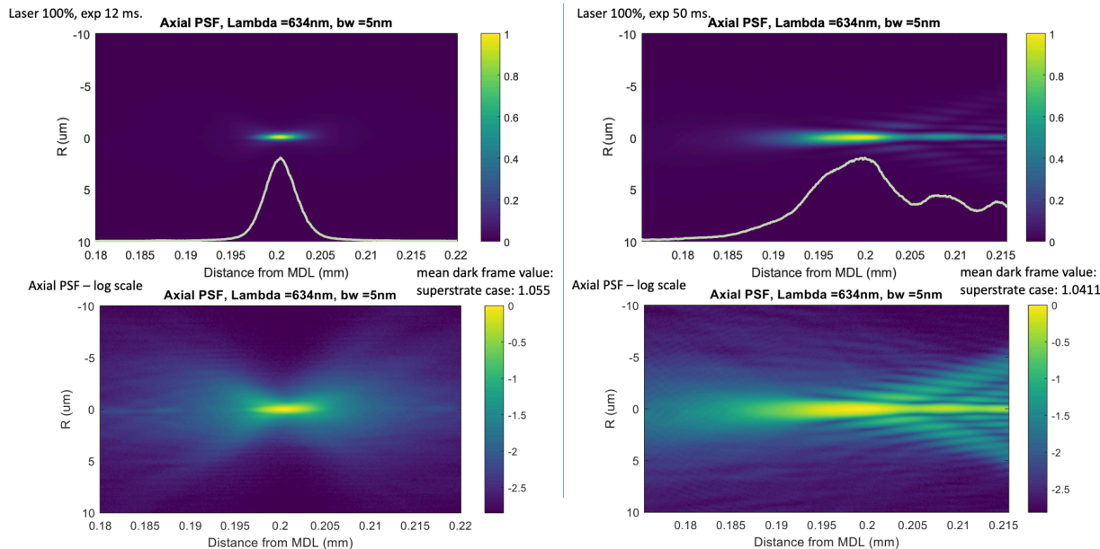
Fig. S7.9 Measured axial PSFs. Scan length: \pm 20 \mu\text{m} on either side of best focal plane, Total length = 40 \mu\text{m} , Step size = 0.1 \mu\text{m} , Number of steps = 400, \lambda = 634 \text{ nm} , \text{bw} = 5 \text{ nm} (set using VARIA).
