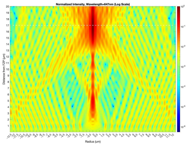
Fig S1.9: Simulated PSF in the XZ plane for the FZP with opaque ring (a) and FZP without opaque ring (b) with diameter = 25 \mu\text{m} , focal length 17 \mu\text{m} , and incidence from air. Note that the efficiency of the FZP without Opaque ring was 15.8379% and with aperture was 15.4457%
