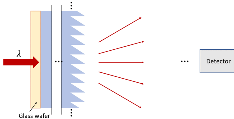
Fig. S2.2: Schematic diagram showing practical use case of the “infinite superstrate” type grating structure.
